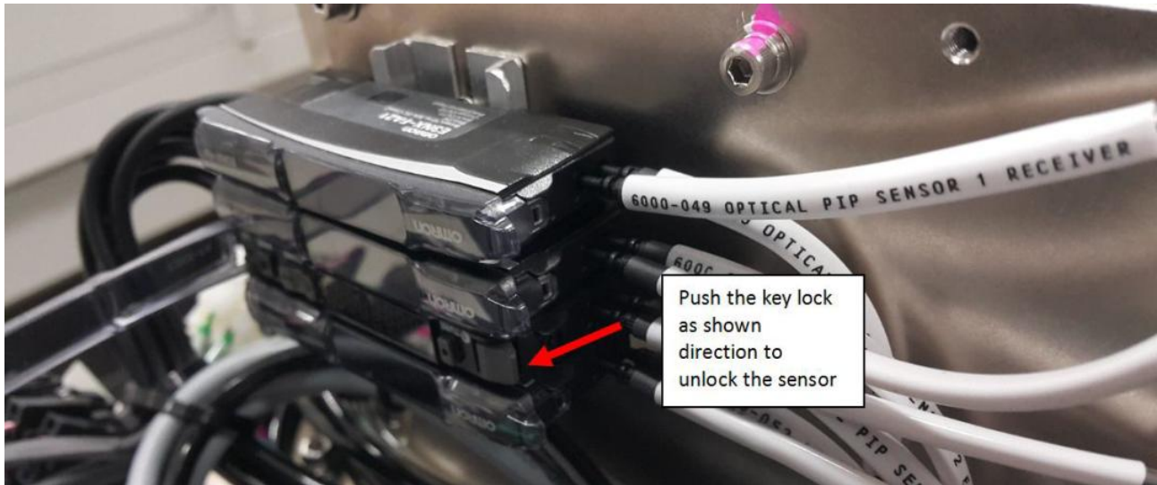
Figure 12 Sensor Amplifier
