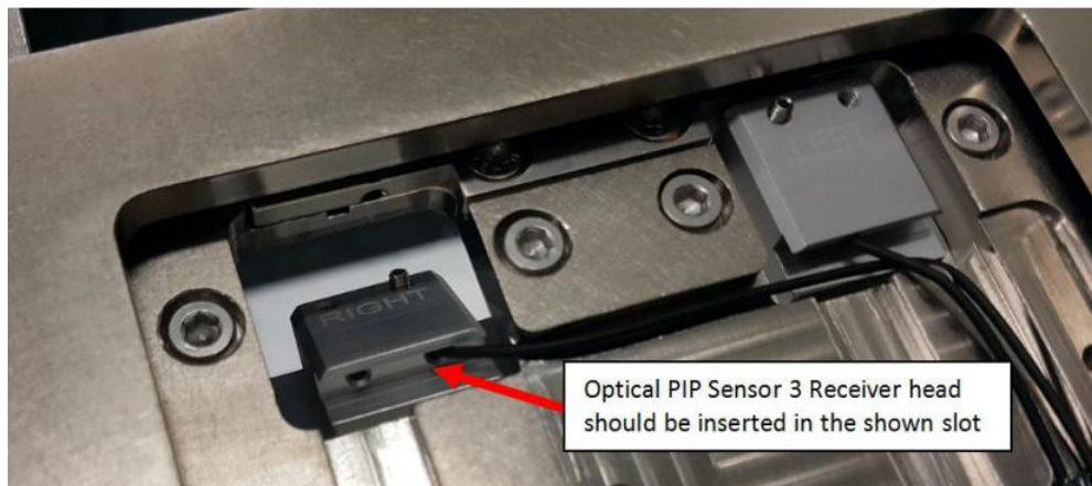
Figure 37 Sensor Receiver 3
