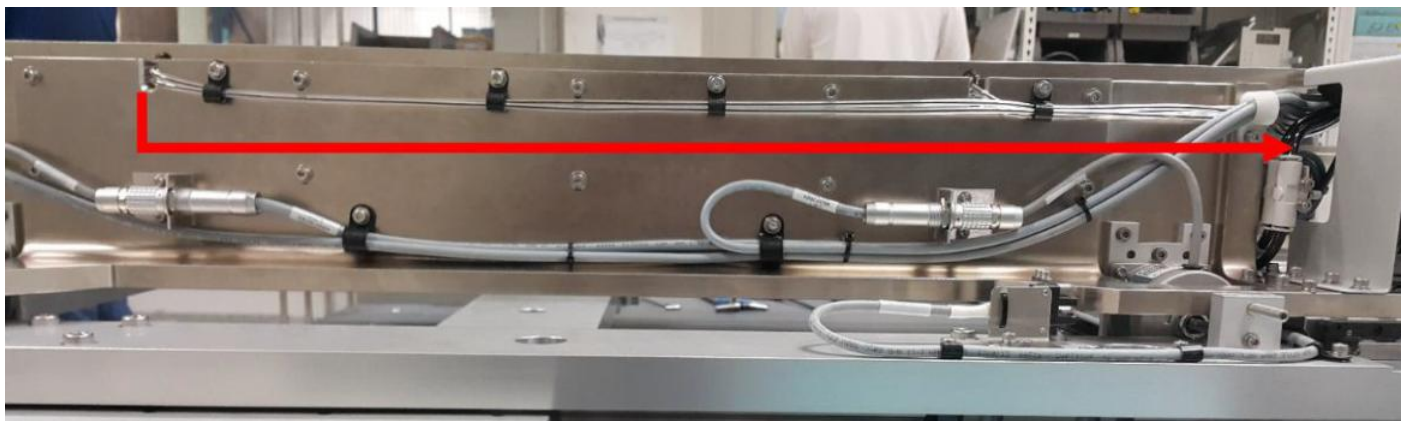
Figure 8 sensor 3 Emitter Cable Routing
