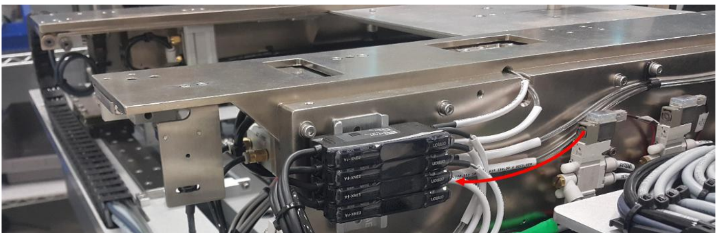
Figure 44 Sensor 3 Receiver Routing
