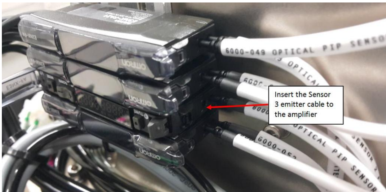
Figure 33 Sensor 3 Emitter Cable
