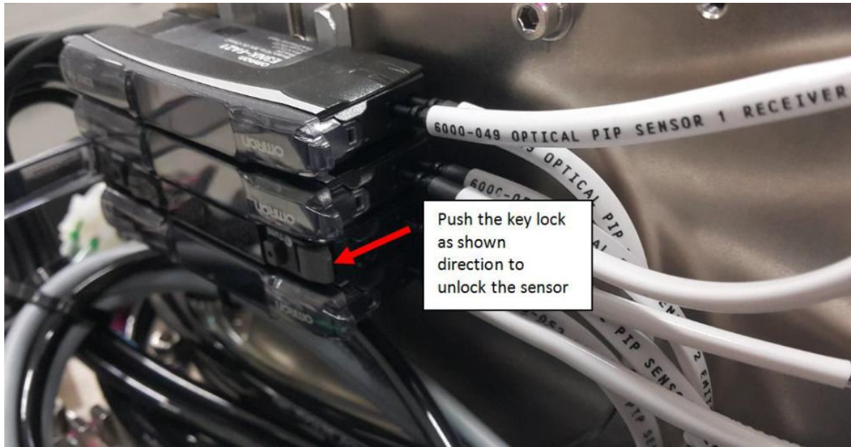
Figure 19 Sensor Amplifier
