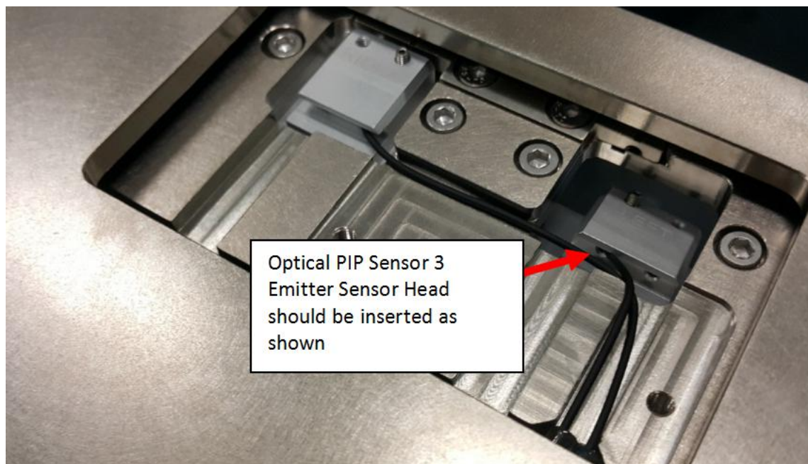
Figure 24 Optical PIP Sensor 3 Emitter Head
