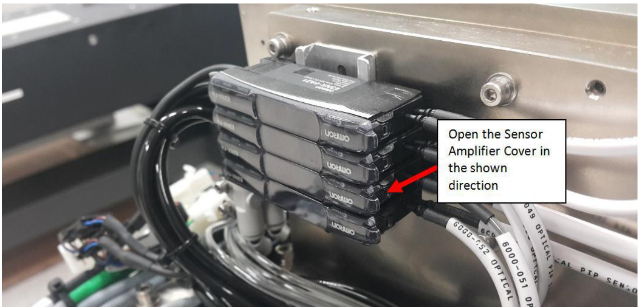
Figure 18 Sensor Amplifier Cover
