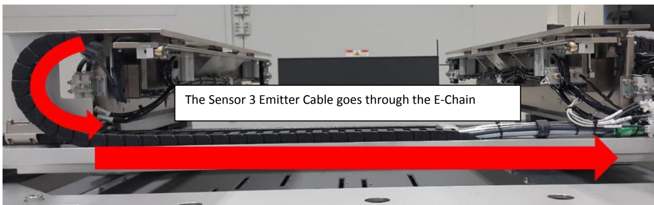
Figure 31 Sensor 3 Emitter (E-Chain)
