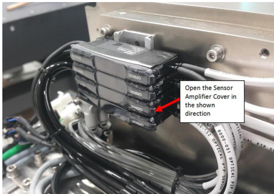
Figure 11 Sensor Amplifier Cover
