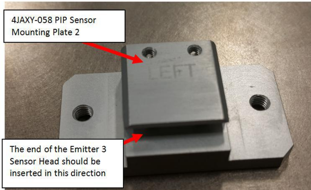
Figure 23 4JAXY-058 PIP Sensor Mounting Plate
