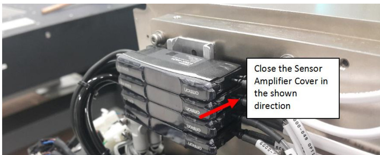
Figure 47 Sensor 3 Amplifier Cover
